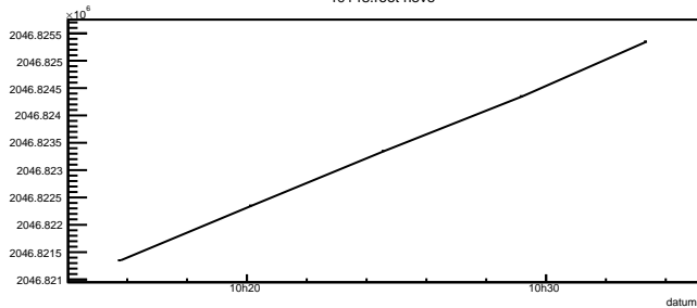
r0148.root 1st anode
