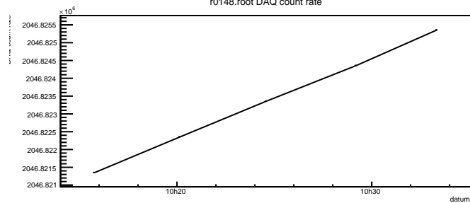
r0148.root DAQ count rate
