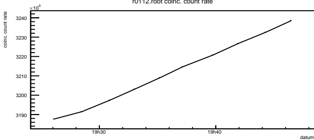
r0112.root coinc. count rate
