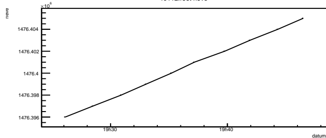
r0112.root 1st anode
