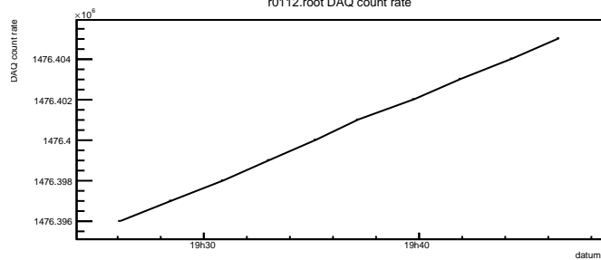
r0112.root DAQ count rate
