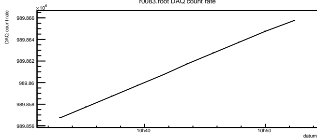
r0083.root DAQ count rate
