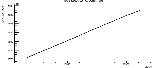
r0083.root coinc. count rate
