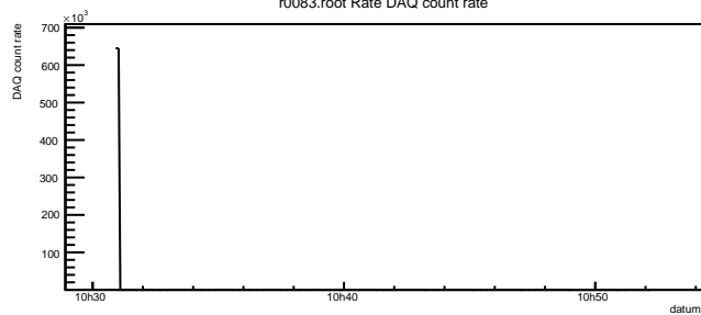
r0083.root Rate DAQ count rate
