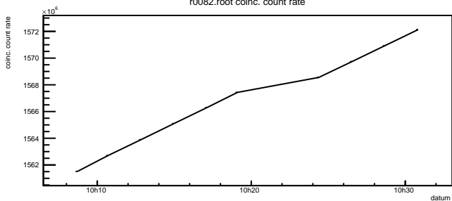
r0082.root coinc. count rate
