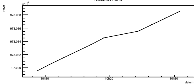
r0082.root 1st anode
