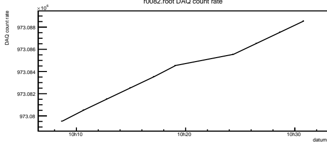
r0082.root DAQ count rate
