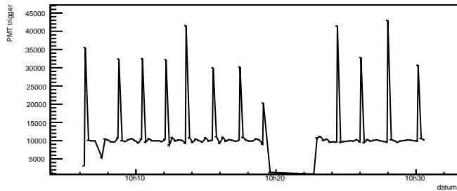
r0082.root Rate 2nd anode
