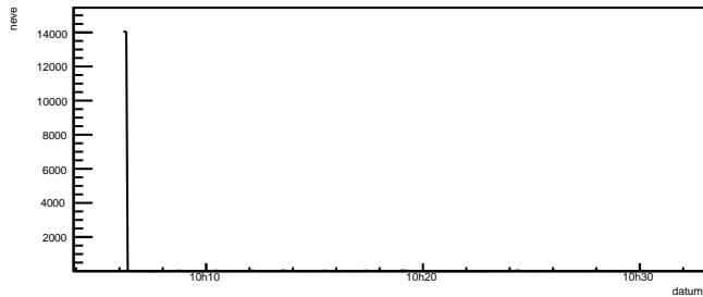
r0082.root Rate 1st anode
