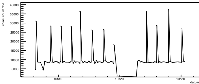
r0082.root Rate coinc. count rate
