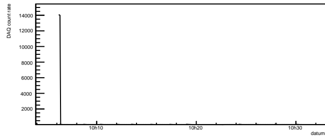
r0082.root Rate DAQ count rate
