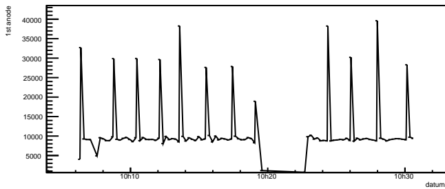
r0082.root Rate coinc. count rate
