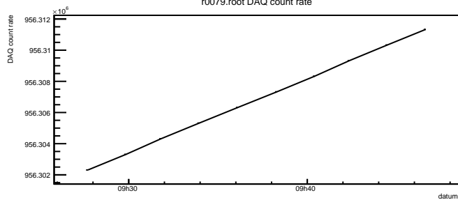
r0079.root DAQ count rate
