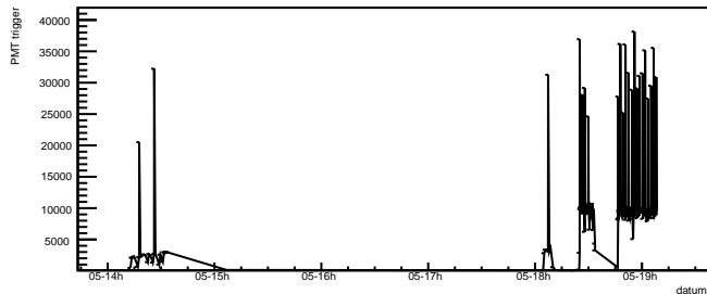
r0067.root Rate 2nd anode
