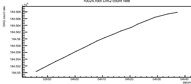
r0024.root DAQ count rate
