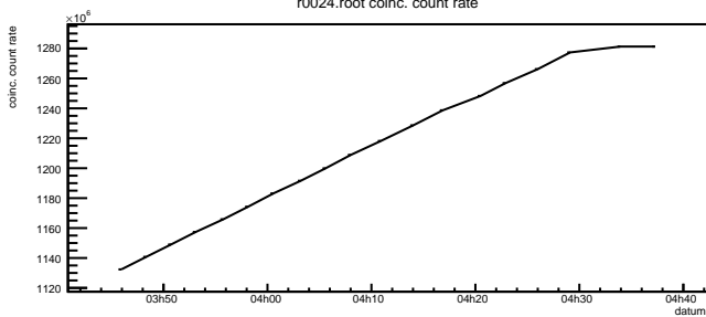
r0024.root coinc. count rate
