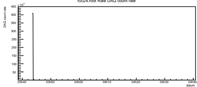
r0024.root Rate DAQ count rate
