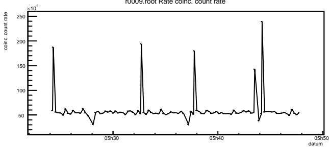
r0009.root Rate coinc. count rate
